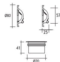
Plastic Recessing Box for Concrete
