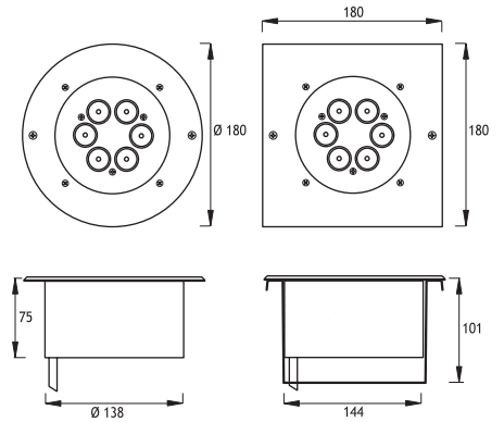
Aluminum recessing tube
