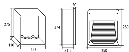
Recessing Box
