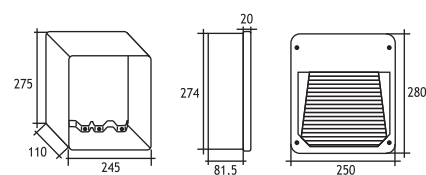
Recessing Box
