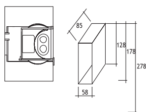
SERIES 106 : IN WALL
