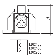
SERIES 206 : IN FALSE CEILING
