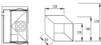
SERIES 104 : IN WALL
