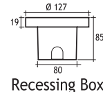
Recessing Box
