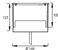
Aluminium recessing tube
