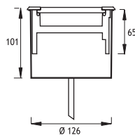
Aluminium recessing tube
